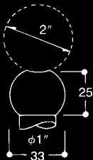
Picket Adapter 919P
