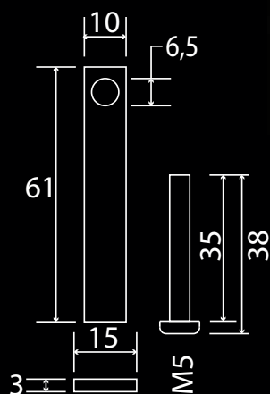
Mini-Rail End Bracket - 660
