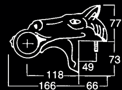
Horse Rail Bracket 992
