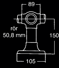
Side Outlet Tee Post 902
