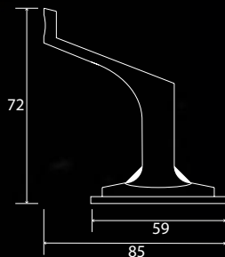
Flat Handrail Bracket 932F
