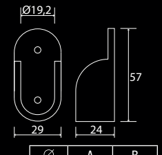
Half Flange I231G
