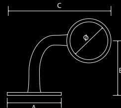
Wall End Bracket
