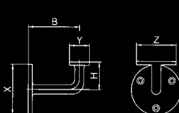
Flat Hand Rail Bracket
