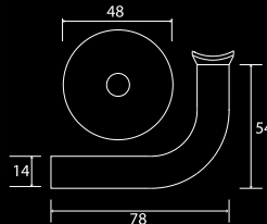
Hand Rail Bracket 860M
