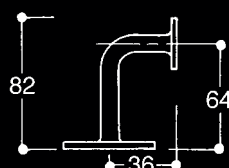
Flat Handrail Bracket 932F
