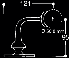
Heavy Duty Handrail Bracket 932H
