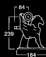
Pegasus Rail Bracket H160
