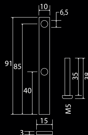
Mini-rail Double Centre Bracket - 671
