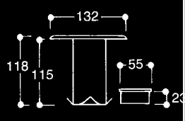
Socket Cap 751 for 2" Tube
