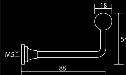
Ball Gond Hook 858
