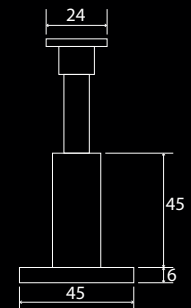
Hand Rail Bracket 860R
