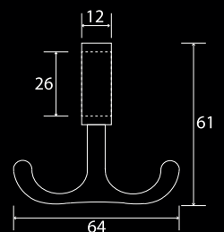
859 Anchor Hook 859CH in chrome
