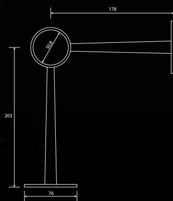
Floor Bracket 979
