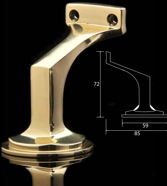
Flat Handrail Bracket 932F
