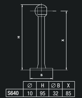
Fiddle End Bracket
