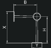
Floor Bracket
