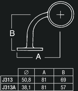
Wall Bracket
