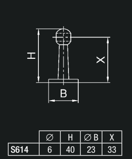
Fiddle Rail Center Bracket
