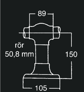
Post Bracket 905
