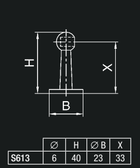
Fiddle Rail End Bracket
