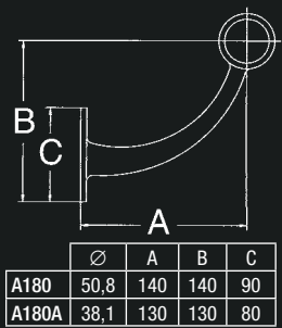
Rail Bracket
