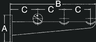
Shelf Support
