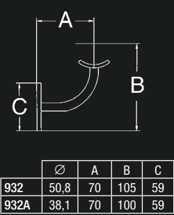
Handrail Bracket
