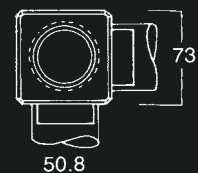
Square Side Outlet Elbow 953SQ
