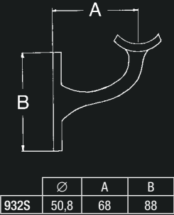
Heavy Handrail Bracket
