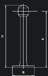
Fiddle Rail Centre Bracket
