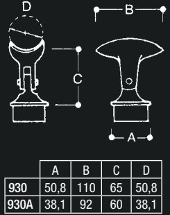
Adjustable Saddle
