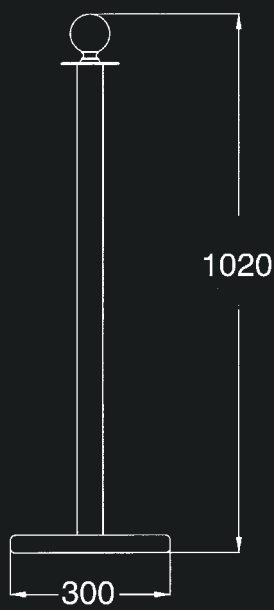
Standard Ball Post 712 & 712CH
