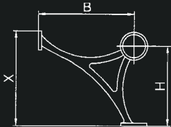
Combination Bracket
