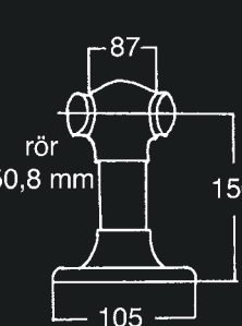
45° Post Bracket 904
