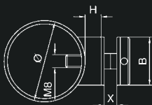
Glass Fittings Adapter
