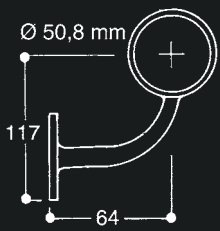
Wall Bracket J314
