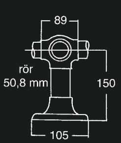
Side Outlet Tee Post 902
