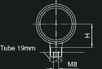
Ball Connection
