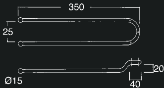
Glass Rack G1930
