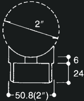
Angle Collar F210
