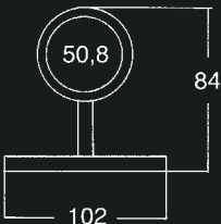
Facia Bracket 991
