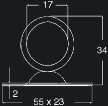
Wall Plate 745
