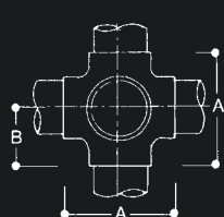
Ball Side Outlet Cross
