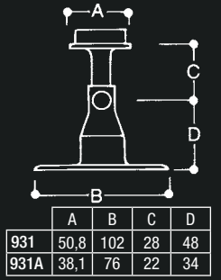
Adjustable Wall Flange
