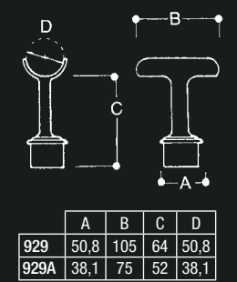
Straight Saddle
