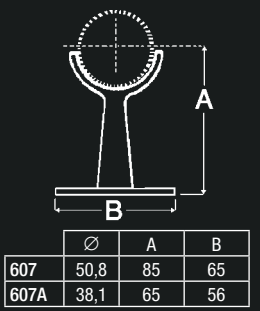
Saddle Post 607
