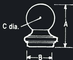
Victorian Stair End
