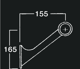
Victorian Bracket 918
