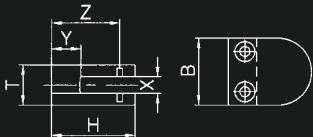
Glass Clip
