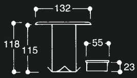
Socket Cap 751 for 2" Tube
