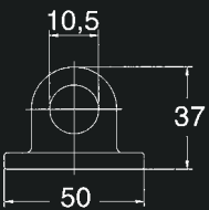
Hook Plate 741
