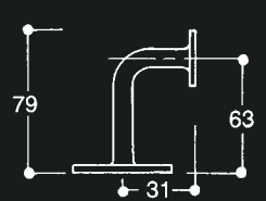
Flat Handrail Bracket 932F
