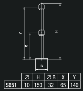
Double Fiddle Rail Centre Bracket
