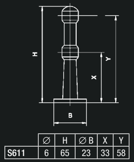
Fiddle Rail Centre Bracket
