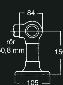
90° Post Bracket 903
