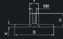
Floor Bracket
