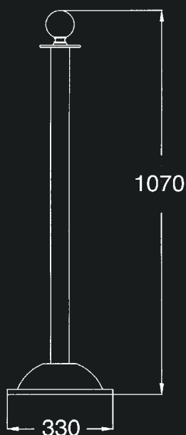
Standard Post 710 & 710CH
