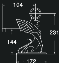
Griffin Rail Bracket 909
