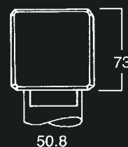
Square Top 948SQ
