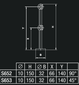
Double Fiddle Rail Elbow Bracket 90°
