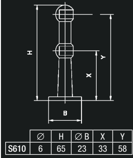
Fiddle Rail End Bracket
