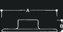
Heavy Duty Floor Flange
