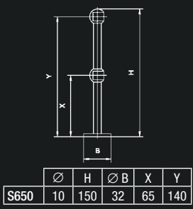
Double Fiddle Rail End Bracket
