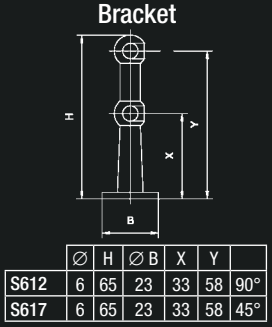
Fiddle Rail Elbow Bracket
