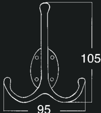
3-Coat Hook 863
