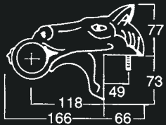
Horse Rail Bracket 992
