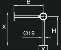
Adjustable Bracket
