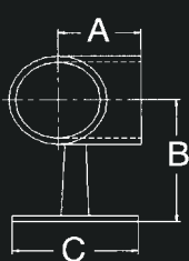
Corner Post
