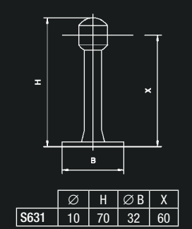
Fiddle Rail Centre Bracket
