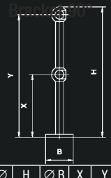
Double Fiddle Rail Elbow Bracket
